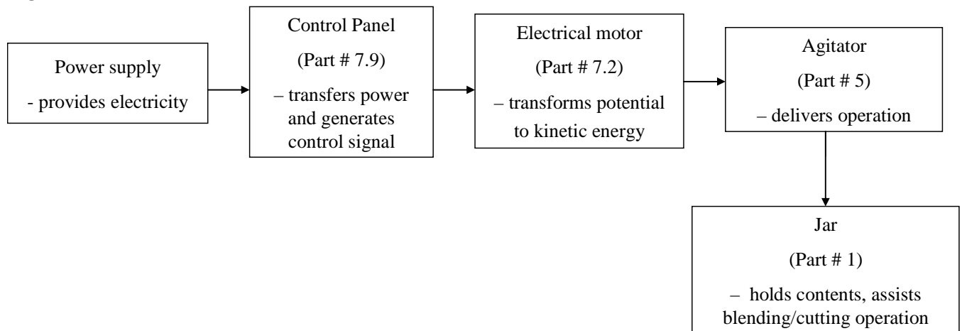
Figure 7: Function Structure
